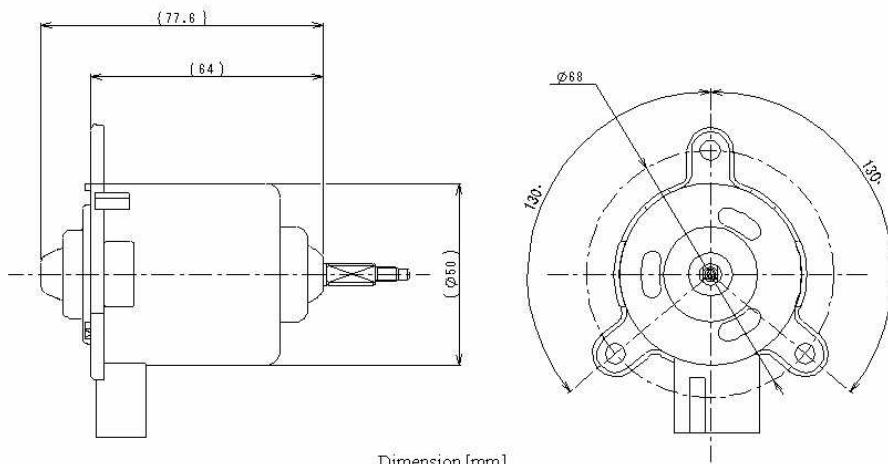
Dimension [mm]
